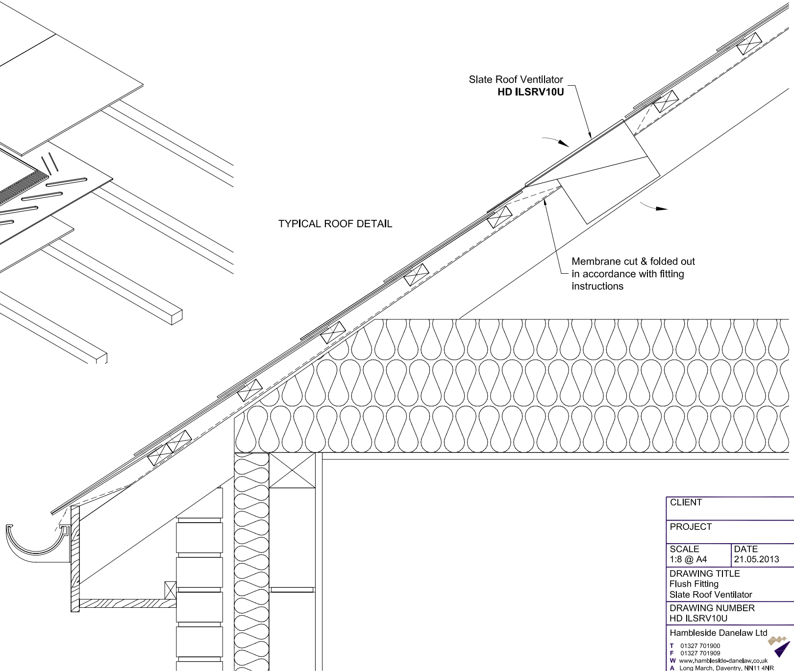
Flush Fitting Slate Ventilator HD ILSRV10U
