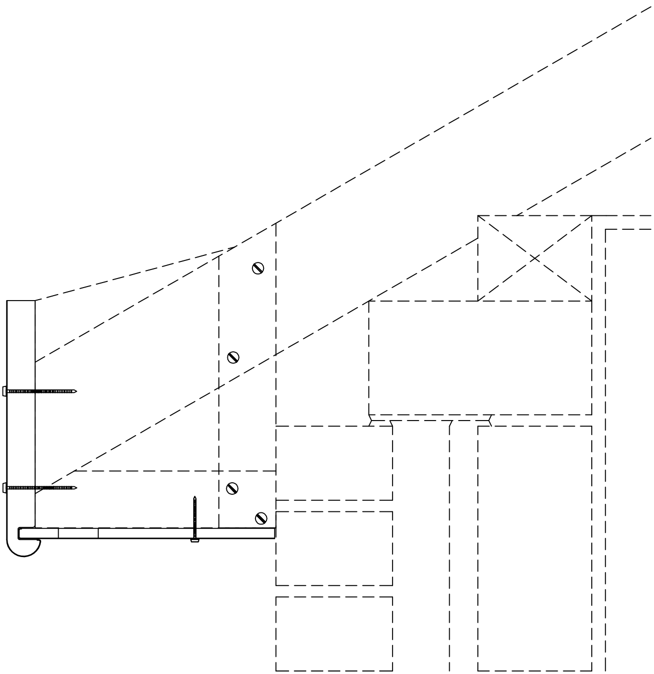
SWISH BUILDING PRODUCTS BULLNOSE JUMBO STANDARD DETAIL SH067Y
