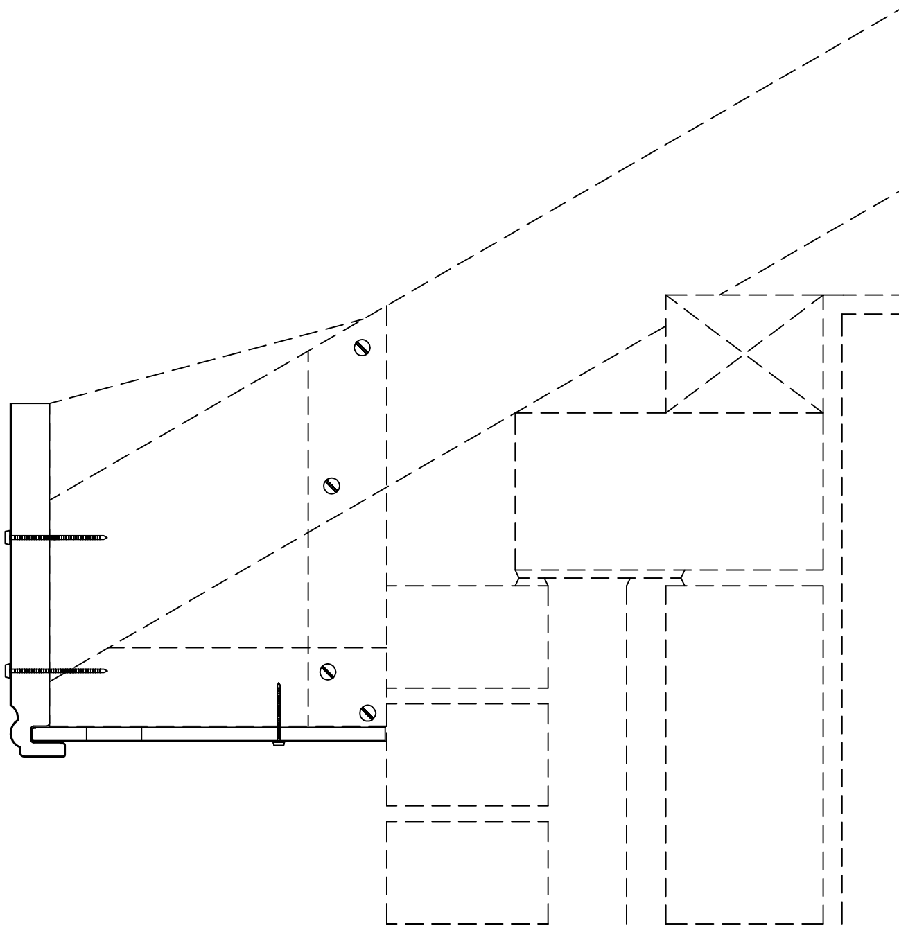
SWISH BUILDING PRODUCTS OGEE JUMBO STANDARD DETAIL SH068Y
