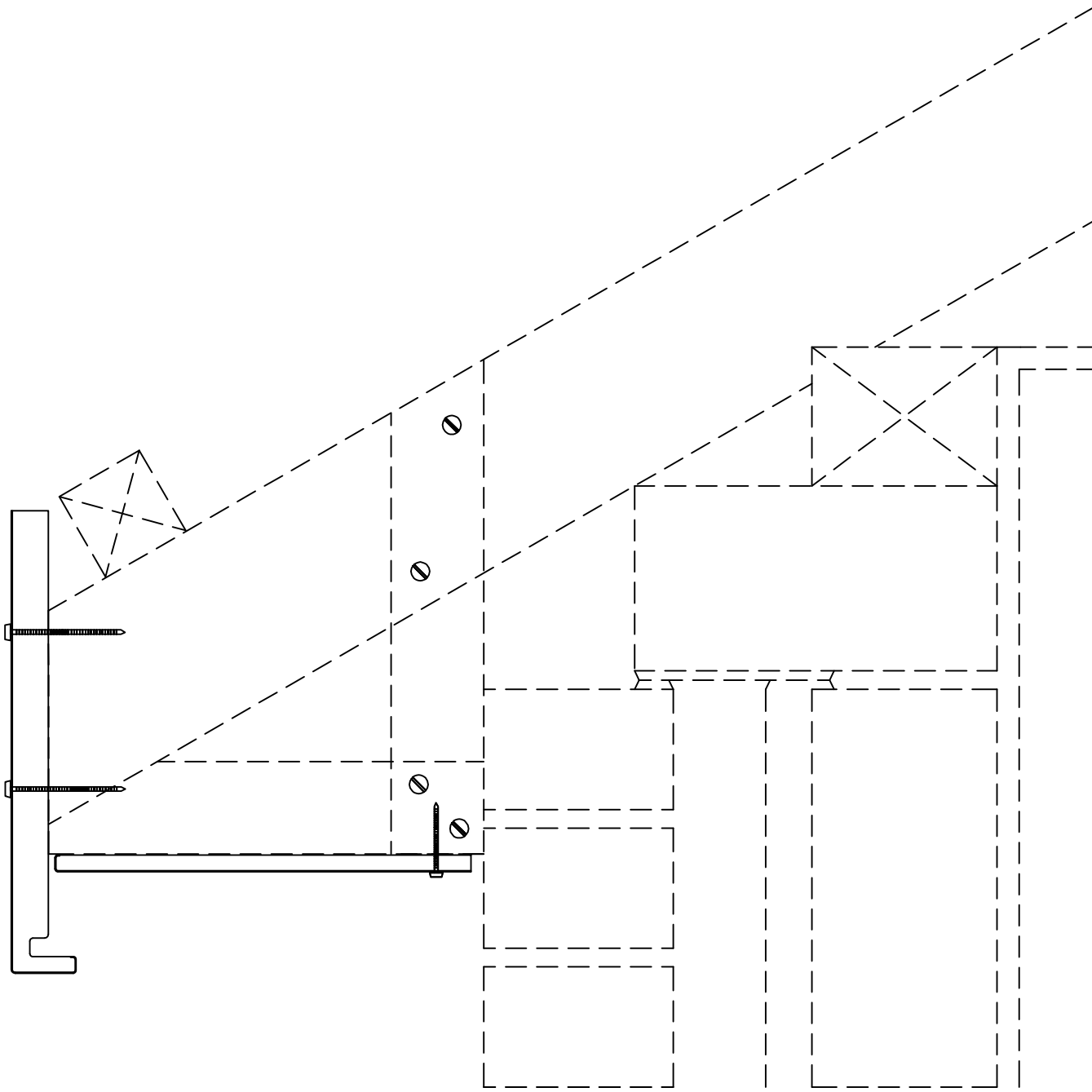
SWISH BUILDING PRODUCTS SQUARE JUMBO RAISED SOFFIT DETAIL SH066Y
