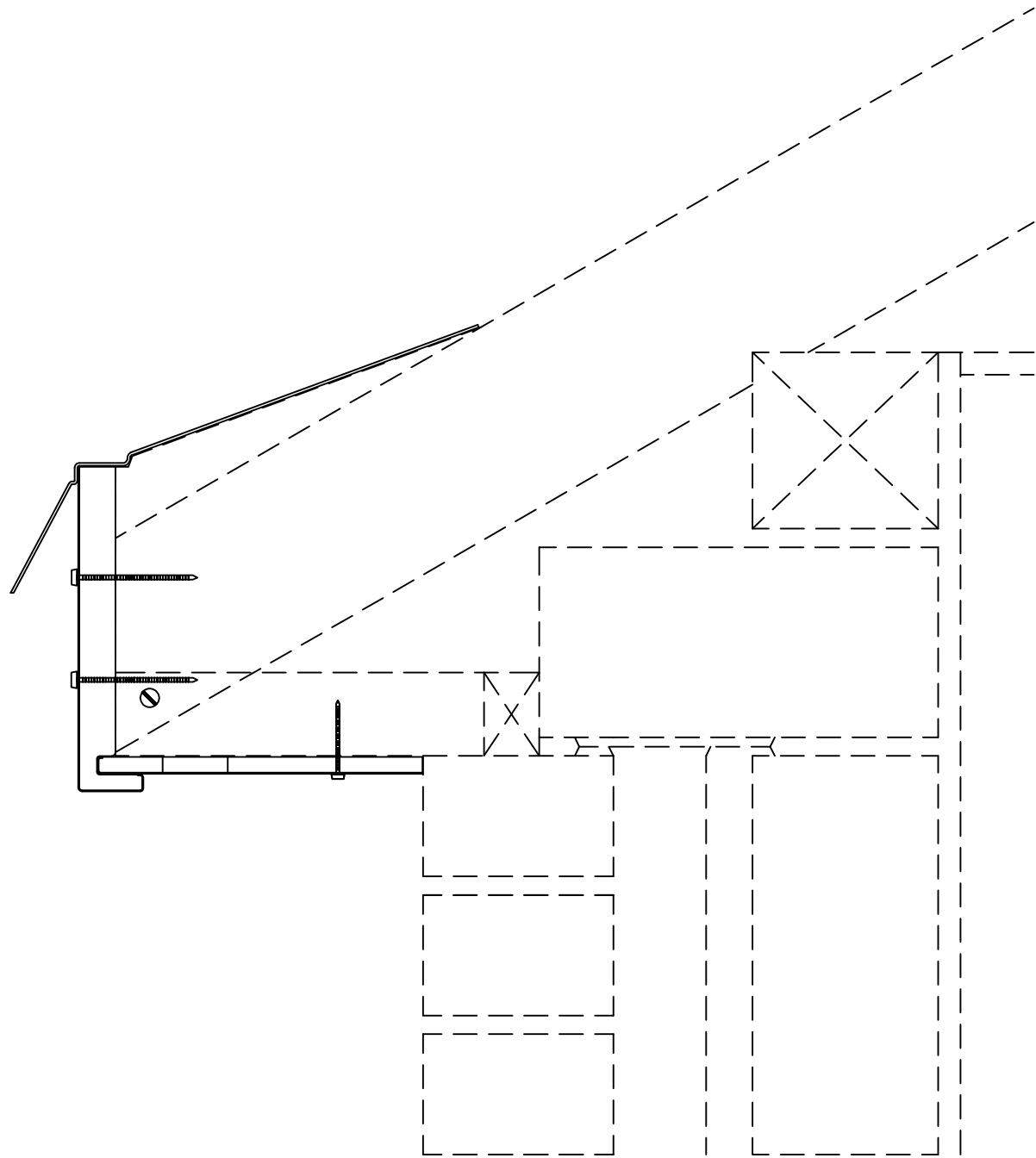
SWISH BUILDING PRODUCTS SQUARE JUMBO STANDARD DETAIL SH065Y
